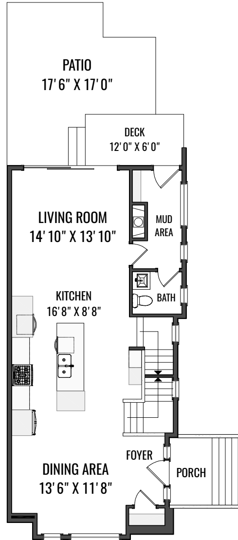
MAIN LEVEL
