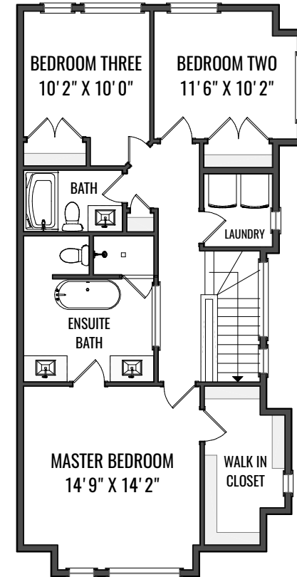
UPPER LEVEL
